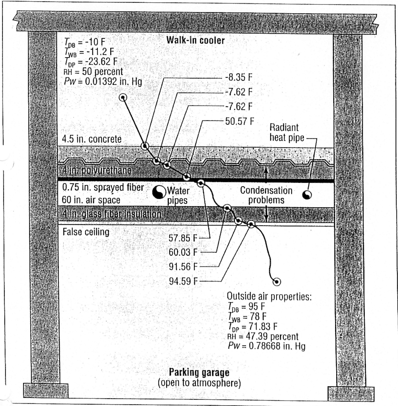
Surface temperatures through the floor along with inside and outside air properties.
